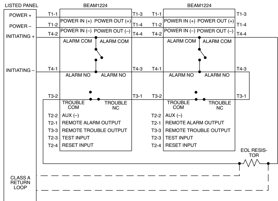
FIGURE 6. WIRING DIAGRAM:
