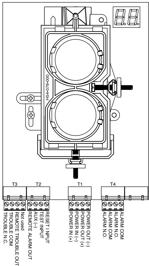
FIGURE 7. WIRING CONNECTIONS AT DETECTOR:
