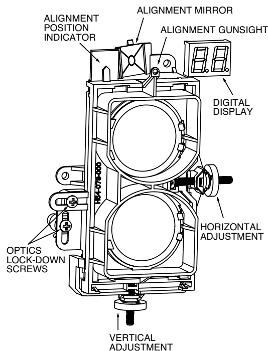
FIGURE 11. ALIGNMENT ADJUSTMENT LOCATIONS:
